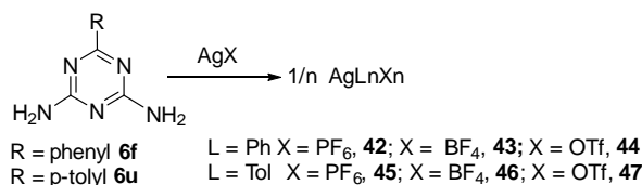
Scheme 7. Self-assembly of silver(I) and diaminotriazines 6f and 6u .
