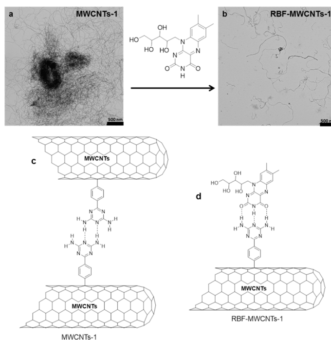
Figure 16. TEM Images of an MWCNTs-1 solution in 1,1,2,2-tetrachloroethane ( 2.5 \cdot 10^{-2} \text{ mg mL}^{-1} ) (a) before and (b) after the addition of an excess of RBF. Expected interaction between MWCNTs-1 (c) before and (d) after the addition of RBF in 1,1,2,2-tetrachloroethane.
