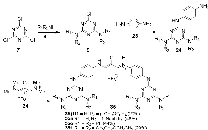
Scheme 4. Synthesis of dimeric triazines 35 with a streptocyanine spacer.
