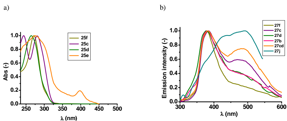
Figure 9. (a) UV spectra of monotriazines 25 , (b) FL spectra of bistriazines 27 .
