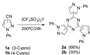
Scheme 1. Synthesis of tris-phenylpyrazolyl-1,3,5-triazines 2a and 2b .
